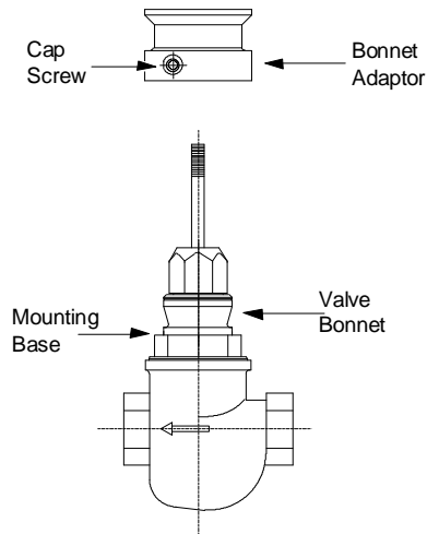
Figure 1: Exploded View of Mounting Kit Assembly to a Honeywell Valve
